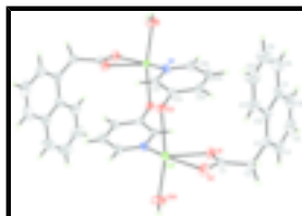
Fig. 1. The structure of the title compound, showing the atomic numbering scheme. Non-H atoms are shown with 30% probability displacement ellipsoids. Unlabeled atoms are related to the labelled atoms by the symmetry operator (1 - x , 2 - y , 1 - z ).
