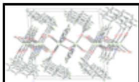
Fig. 2. A packing view of the title compound. The intermolecular hydrogen bonds are shown as dashed lines.
